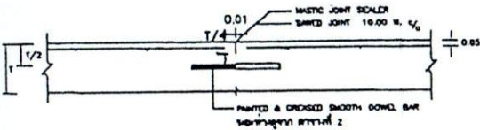
CONTRACTION JOINT
