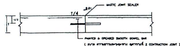
CONSTRUCTION JOINT
