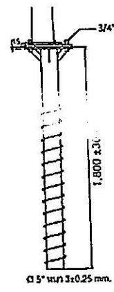
SCREW PILE DETAIL
