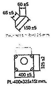
SCREW PILE DETAIL
