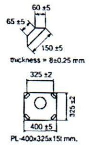
SCREW PILE DETAIL
