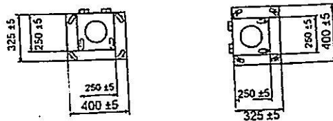
FOOTING DETAIL
